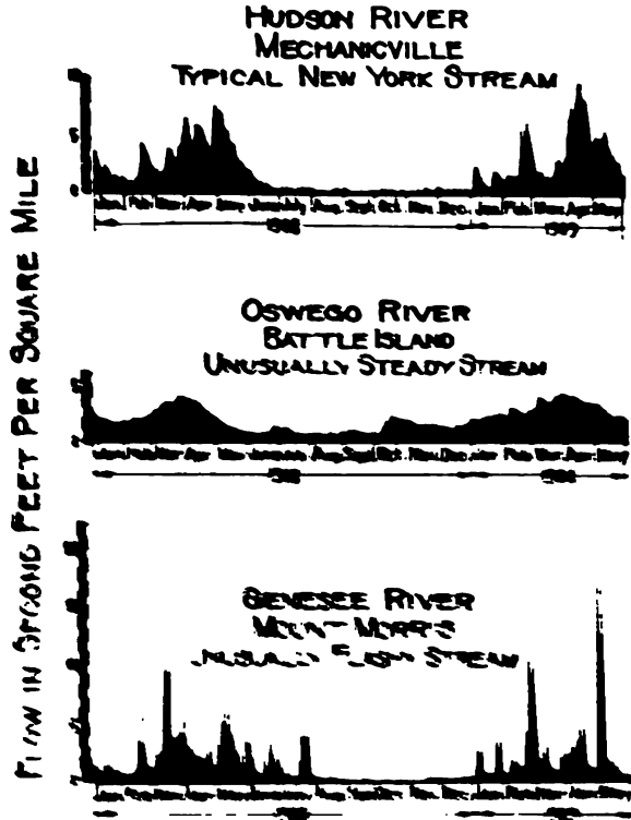
FIGURE 10. Hydrographs showing irregular fluctuations in flow in New York State streams. Courtesy of U. S. Army Corps of Engineers
